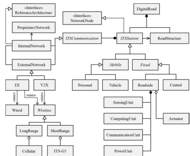
Figure 4: Semantic model of road intelligent transportation systems
