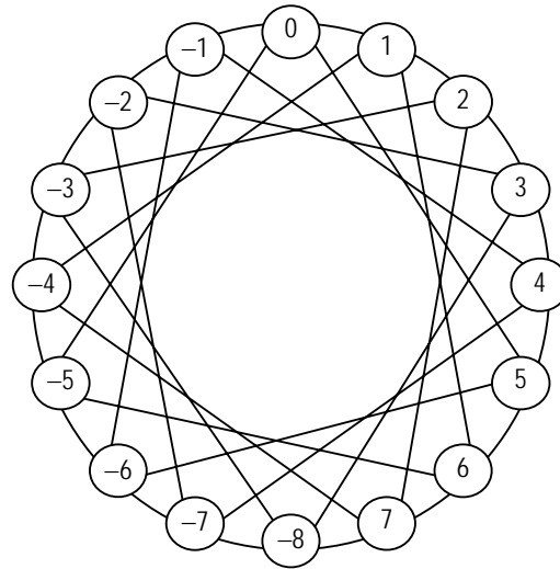
Figure 7. The chordal ring network CR(16; 5) with 16 nodes and chord length 5
